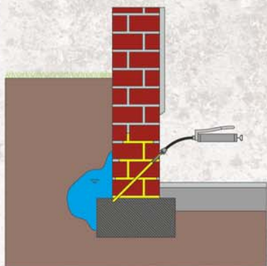
Effectiveness of a horizontal barrier
